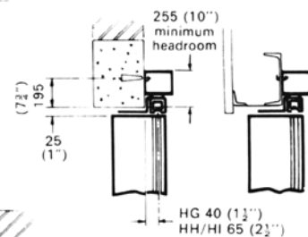
Alternative Section through Head
