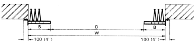
Plan Bi-Parting Doors
