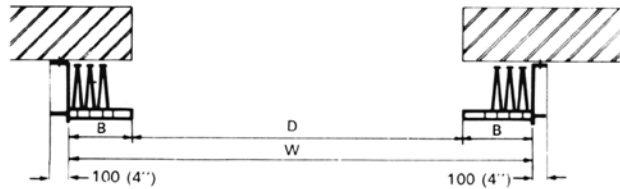
Plan Bi-Parting Doors
