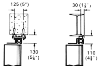
HH & HI details only
